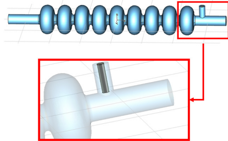
Figure 4: The TESLA cavity with the Stanford/Rossendorf coupler shown lowermost.
