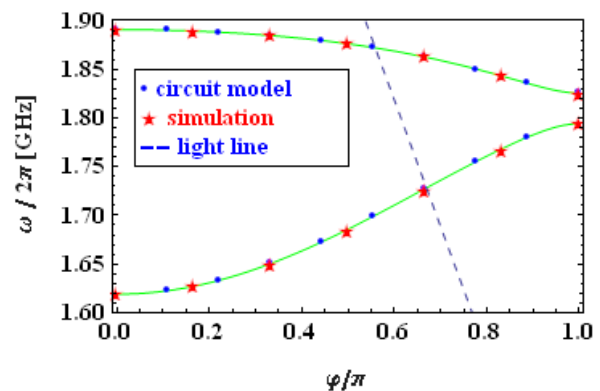
Figure 1: Dispersion curves for the first two dipole bands of a TESLA cavity from a two-band circuit model.
