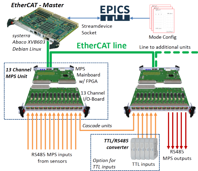
Figure 5: Machine Protection System core components.
