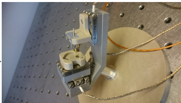
Figure 3: XYZ-control through nm resolution linear piezo stages and tungsten tip.
