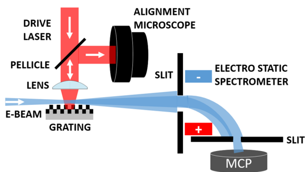
Figure 2: Design scheme of the DLA test setup. The electron beam is emitted from a SEM and is then subsequently passing the acceleration grating and an energy spectrometer.
