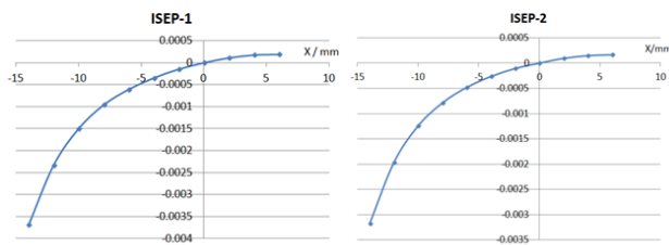
Figure 7: Field uniformity of the two septum magnets.
