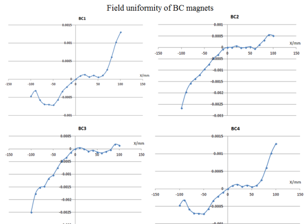
Figure 2: Field uniformity of the four BC magnets.
