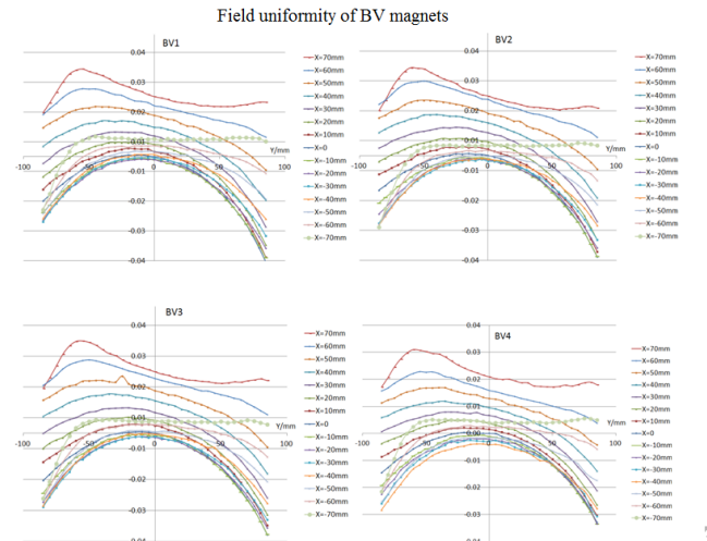
Figure 5: Field uniformity of the four BV magnets.
