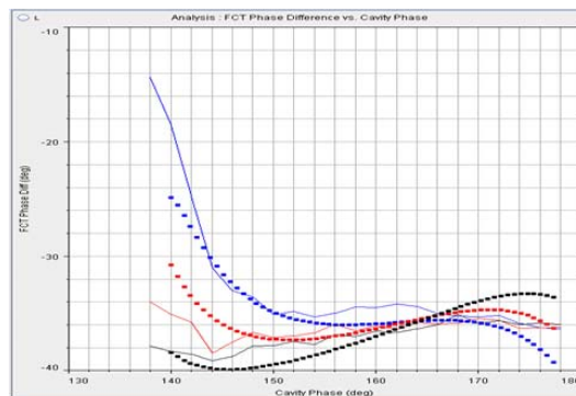
Figure 7: Plots of the DTL tank1 phase scan. Plotted are experimental data (solid lines) and simulation results (solid circles) for three different RF amplitudes.
