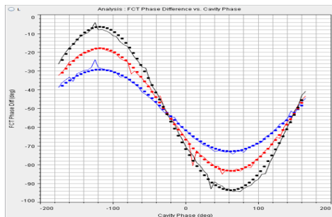
Figure 6: Measured phase differences (degrees) between two FCTs as functions of the buncher02 cavity phase. Plotted are experimental data (solid lines) and simulation results (solid circles) for three different RF amplitudes.
