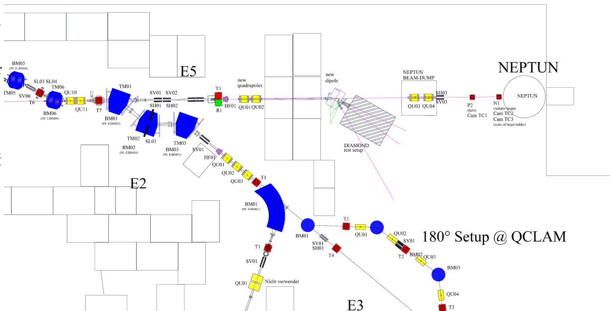
Figure 4: Floor-plan of the E5 beam line of the S-DALINAC. A dipole magnet will be installed and a pair of quadrupoles in order to focus the beam on the diamond detector setup.
