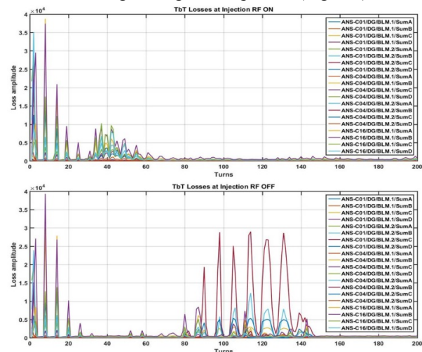
Figure 12: a and b losses measurement (turn by turn data) at injection with RF ON (top) and OFF (bottom).
