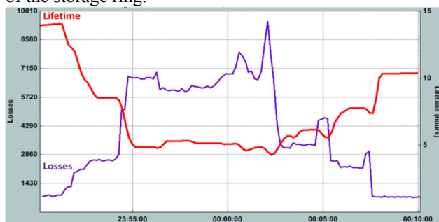
Figure 14: Correlation between losses measurement in slow mode and the beam lifetime.
