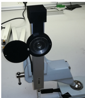
Figure 6: Cesium source positioning on the BLM with a 3D printed support (in black).
