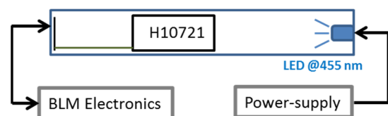
Figure 3: Setup for the calibration with a LED (diode).
