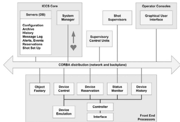
Figure 4: ICCS CORBA Distributed Framework.
