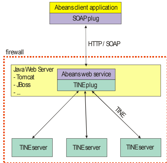
Figure 2: Architecture of Abeans Web Services
