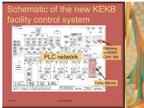
Figure 1: Schematic of the new KEKB facility control system
