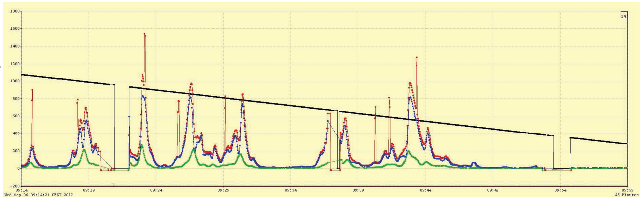
Figure 7: Radiation profile measured with the Pandora device alongside the XFEL accelerator (test run between the two docking stations at 1069 m and 280 m, black: robot position [m], red: dose rate [µSv/h], blue: averaged gamma dose rate [µSv/h], green: averaged neutron dose rate [µSv/h], missing data: wireless data connection temporarily lost)
