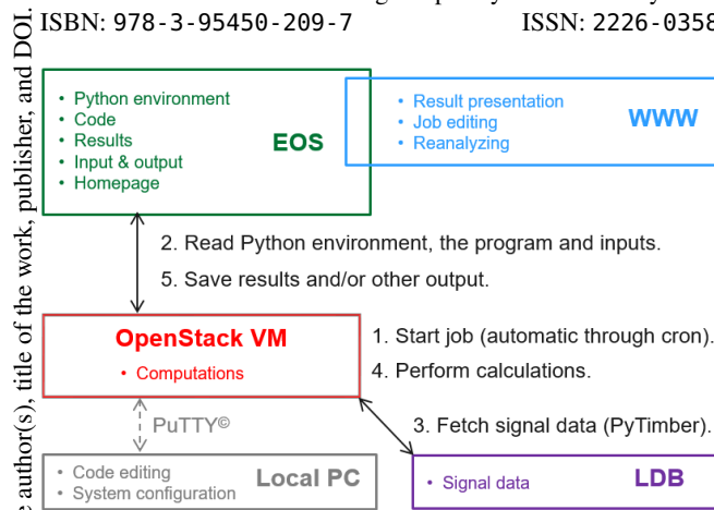
Figure 2: Schematic over the technical infrastructure set up to for the project and its work flow.
