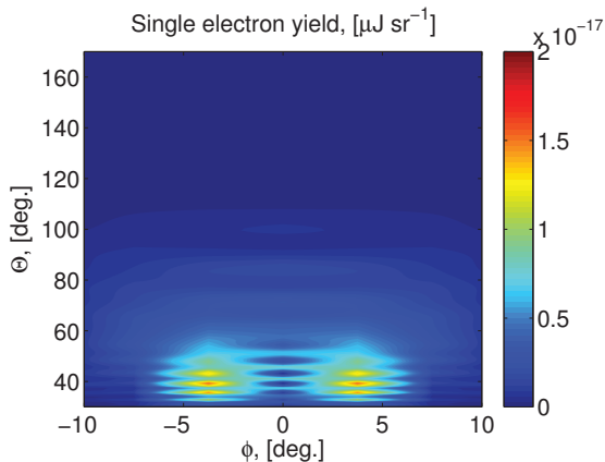
Figure 2: SEY for SP effect. Grating 40 \times 180 \text{ mm}^2 with 8 mm pitch and 30^\circ blaze angle.
