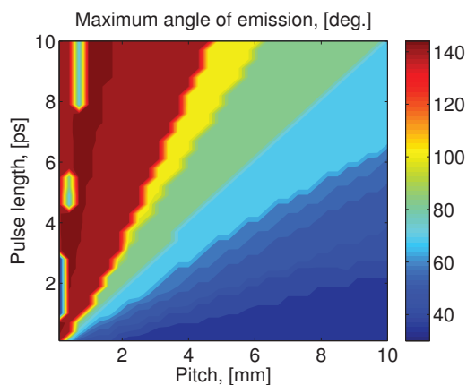
Figure 4: Maximum angle of emission for SP effect as function of pulsewidth and grating pitch. Grating 40 \times 180 \text{ mm}^2 with 30^\circ blaze angle. The beam-grating separation is 3 mm.
