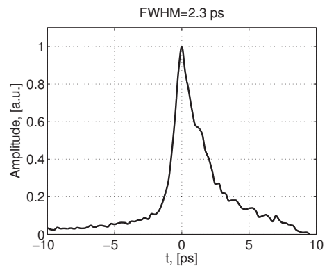
Figure 8: Profile of the bunch at the exit of the CLIO accelerating section (see [5]).
