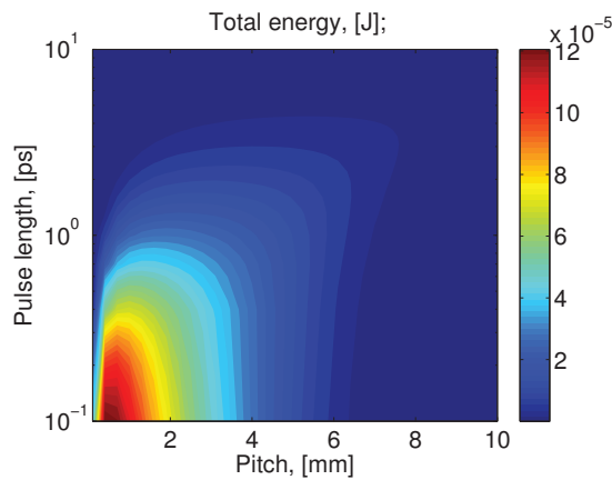
Figure 5: Total energy for SP effect presented as function of pulsewidth and grating pitch. Grating is 40 \times 180 \text{ mm}^2 with 30^\circ blaze angle.
