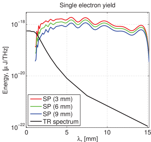
Figure 1: Single electron yield for TR and SP. The screen diameter for TR is 40mm. SP SEY is presented for different beam-grating separation (3 mm, 6 mm and 9 mm). The grating used here is 40 \times 180 \text{ mm}^2 with 8 mm pitch and 30^\circ blaze angle.
