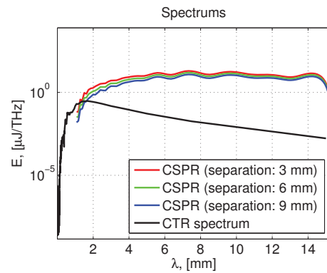
Figure 9: CSPR and CTR energy density as function of wavelength. The CSPR spectrum is presented for beam-grating separations of 3 mm, 6 mm and 9 mm. The grating dimensions are 40 \times 180 \text{ mm}^2 with 8 mm pitch and 30^\circ blaze angle. The screen diameter for TR is 40 mm. The signal is measured as integrated with a 50 mm diameter parabolic mirror located 300 mm from the beam axis.
