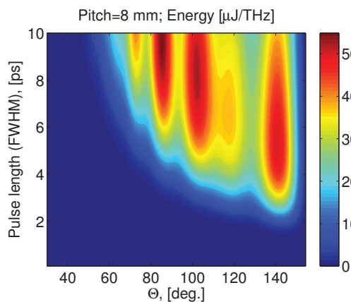
Figure 6: Evolution of the CSPR spectrum with a constant grating pitch and a wavelength changing with the angle. The grating dimensions are 40 \times 180 \text{ mm}^2 with 8 mm pitch and 30^\circ blaze angle.
