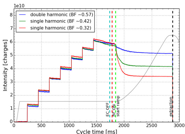
Figure 2: Beam intensity along the LEIR magnetic cycle (B field in gray) for three different values of bunching factor (BF).
