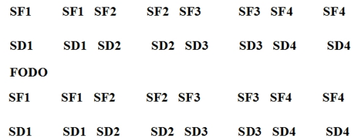
Figure 6: Sextupole scheme of CEPCB.
