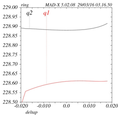
Figure 7: Tune as a function of energy spread.
