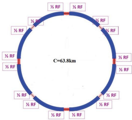
Figure 2: Layout of CEPCB.
