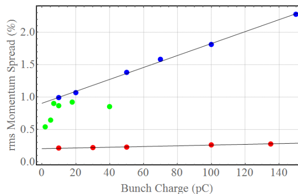
Figure 2: Momentum spread vs charge in spectrometer (red), BA2 (blue) and BA1 (green).
