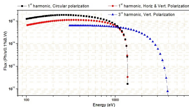
Figure 1: Tuning curves of the helical undulator source of SM, into central radiation cone. linear polarization: 1 st and 3 rd harmonics, circular polarization: 1 st harmonic
