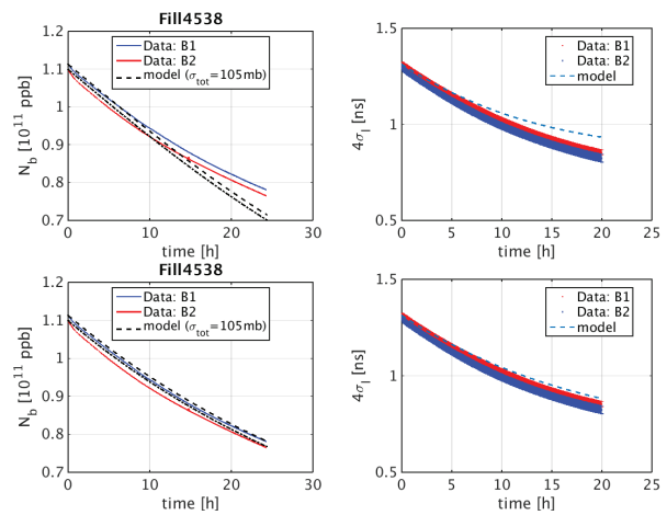
Figure 3: Data to model comparison of the bunch current (left) and bunch length (right) evolution. On top the transverse emittance used is the one predicted by the luminosity model, while on the bottom the transverse emittance used is the one from the BSRT data.
