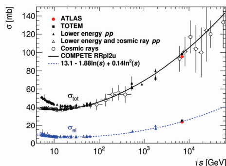
Figure 1: Dependences of total, inelastic and elastic cross-sections on the scattering energy \sqrt{s} [7].
