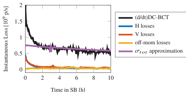
Figure 4: Instantaneous losses during Stable Beams for an example fill of 2015.
