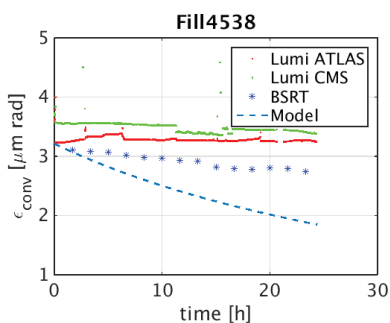
Figure 2: Emittance evolution during collisions, for a typical fill from 2015, from ATLAS luminosity (red), from CMS (green), from the BSRT data (blue stars) and the model prediction (blue dashed line).
