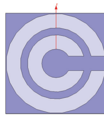
Figure 5: Geometry of the Optimised Unit-Cell.
