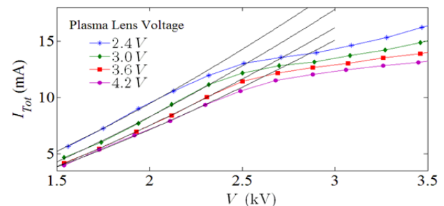
Figure 1: Perveance plot of a 30 keV H - beam for various plasma lens voltages. The arc current was set at 20 A and 130 V and the gas flow was set a 15 sccm. The data was fitted with the 3/2 power law over the extraction limited region.
