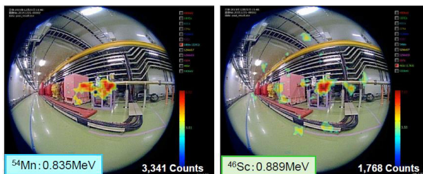
Figure 7: Images for 54 Mn and 46 Sc (0.889 MeV).
