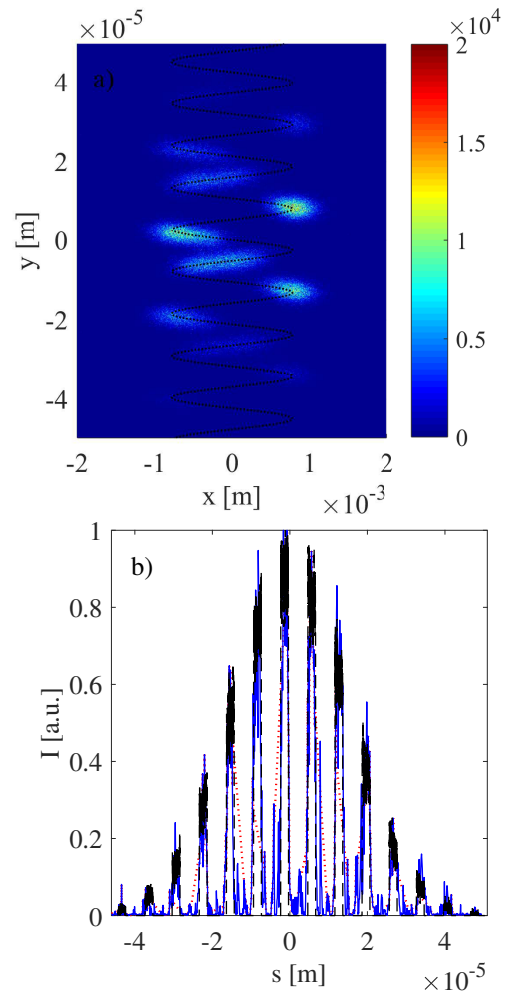
Figure 2: Reconstruction of an electron beam of 15 \mu\text{m} rms length consisting of 2 \mu\text{m} long microbunches at 5 \mu\text{m} distance. The reconstructed values are 15.55 \mu\text{m} for the full rms beam length, 1.94 \mu\text{m} for the microbunch length and 5.00 \mu\text{m} for the average microbunch distance. a): transverse beam distribution at the imaging screen with a sinusoidal fit overlaid; b): original beam distribution (black) and recovered profiles based on a single sub-fs diagnostic measurement (dotted red) and five measurements with slightly varying laser phase (solid blue).
