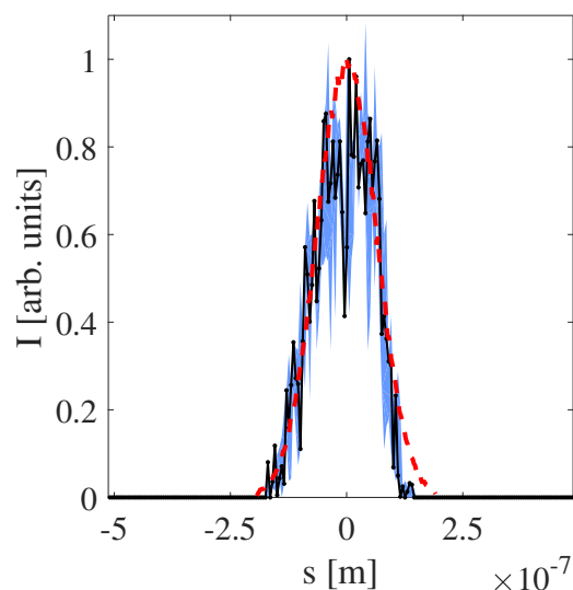
Figure 3: Reconstructed SINBAD beam with an rms beam length of 6.03 \times 10^{-8} m (solid black) overlaid by the normalised initial beam profile (dashed red). The blue region shows the profile error, estimated based on the uncertainty in the fitting coefficients of the reconstruction algorithm.
