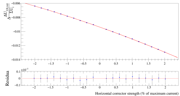
Figure 8: The relative vertical voltage ratio in dependency of the applied horizontal bump strength.
