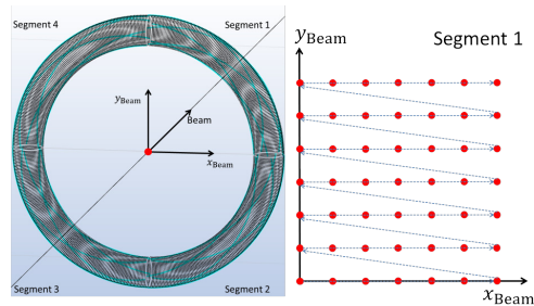
Figure 2: Simulation setup and applied beam positions. On the left hand side the model setup for the numerical simulation is presented. The beam is moved to defined positions in the horizontal and vertical plane, which is illustrated on the right hand side.
