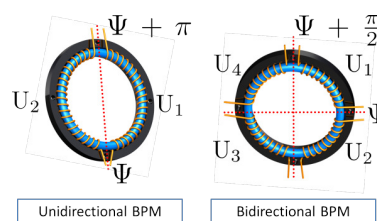
Figure 1: The halved Rogowski coil can determine a beam displacement in one direction, whereas the signals of the individual quarters in the configuration on the right hand side can be combined to yield information about displacements in both directions.
