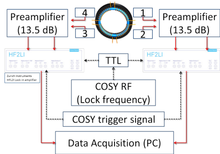
Figure 5: Readout scheme of the Rogowski coil BPM.
