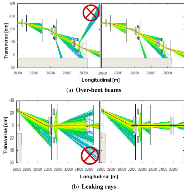
Figure 7: Patching two weaknesses in HXR at BTH. “⊗” mark un-allowed trajectories.
