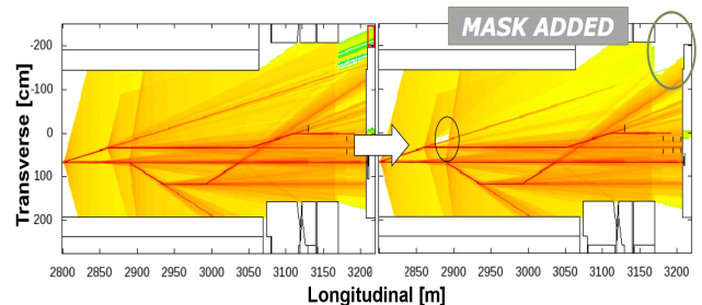
Figure 4: Ray-trace for LCLS-II beam-lines in BSY: (left) without BCS shielding; (right) after adding a small mask.
