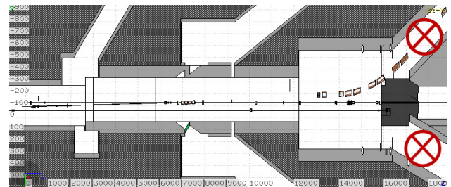
Figure 3: Top view of SLAC Linac sector 28 through BSY and west area of BTH. High power LCLS-II beams mis-steered towards ES-A or ES-B should be intercepted.
