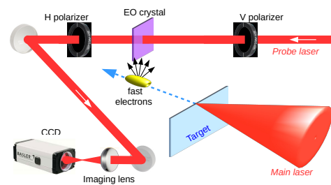
Figure 1: Setup of the experiment. The FLAME laser is focused on a metallic target from where fast electrons can escape. The EOS system, based on a 500 \mu m thick ZnTe crystal placed 1 mm downstream the target, allows to measure the temporal profile of the emitted electrons by means of an ancillary laser beam probing the local birefringence induced by the electric field.
