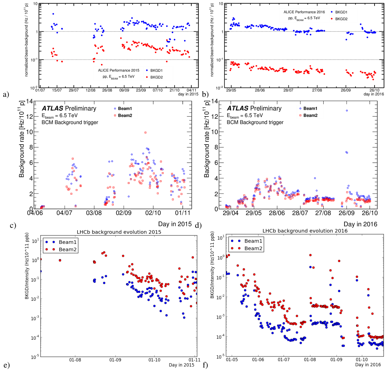
Figure 2: Beam-induced background evolution during 2015 (left) and 2016 (right) for ALICE (upper), ATLAS (middle) and LHCb (lower).
