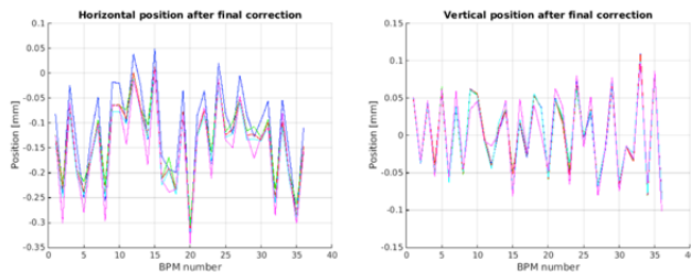
Figure 12: Sets of horizontal and vertical closed orbits after automatic orbit correction at final energy.
