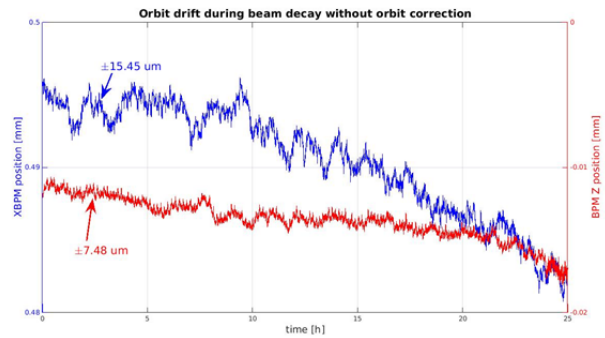
Figure 8: The vertical position drift of electron (red) and photon (blue) beam monitored over 25h without orbit correction.
