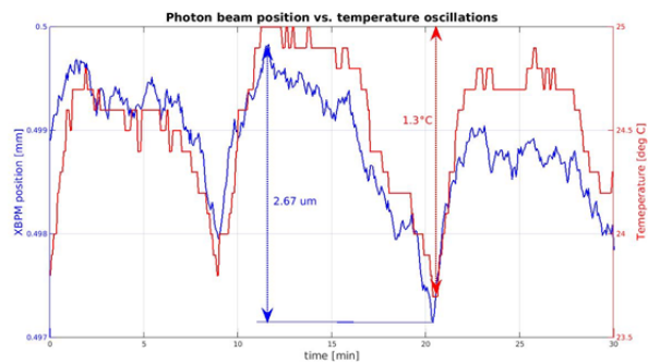
Figure 9: The temperature (red) and the photon beam oscillations monitored over 30 min with applied orbit correction.
