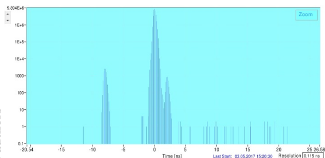
Figure 2: Bunch population after clearing of spurious bunches.
