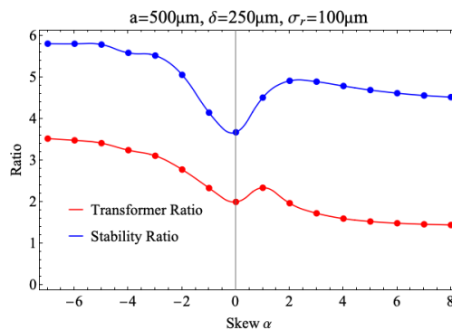
Figure 7: The transformer and stability ratio for increasing skewness, for a bunch with \sigma_t = 3 ps.
