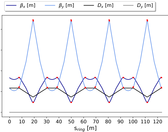
Figure 2: Optics of the chosen working point. The x-axis shows the position inside the storage ring and the y-axis shows the magnitude of the individual properties. Location of quadrupoles are marked with red dots.
