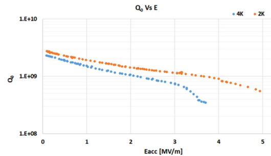
Figure 10: Q curve from the rf testing.
