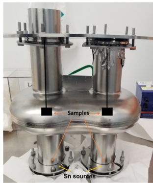
Figure 6: Twin cavity #1 setup for coating (top) and tin sources (bottom).
