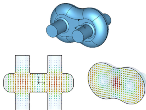
Figure 1: Twin axis cavity model (top) and electric (left) and magnetic (right) field profile at the twin cavity cross section (bottom) from CST microwave studio [3].
