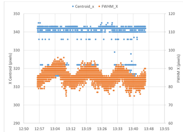
Figure 4: Electron beam spot size and position jitter on YAG screen.
