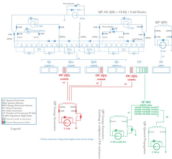
Figure 1: IT String circuit layout.
