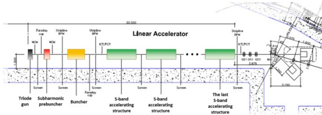
Figure 3: Components of the SPS-II 150-MeV linac.
