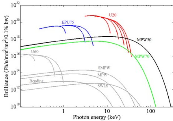
Figure 2: Calculated brilliance of SPS (grey) and SPS-II sources.
