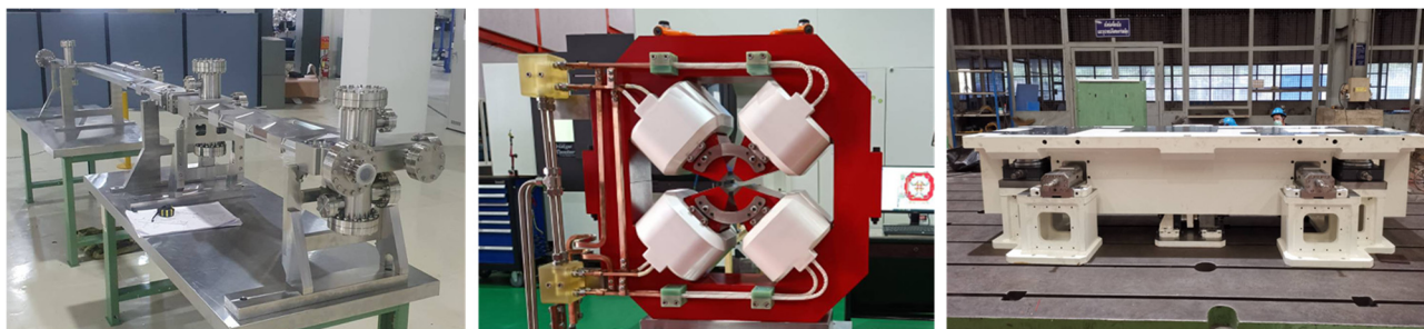
Figure 7: Prototype of vacuum chambers, magnets, and girders for the half-cell of DTBA lattice.
