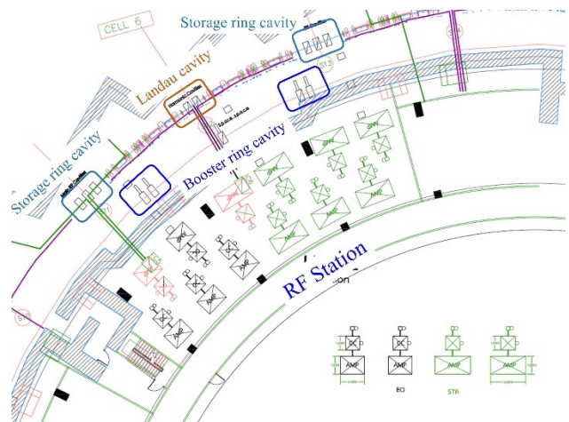
Figure 4: RF system of SPS-II.
