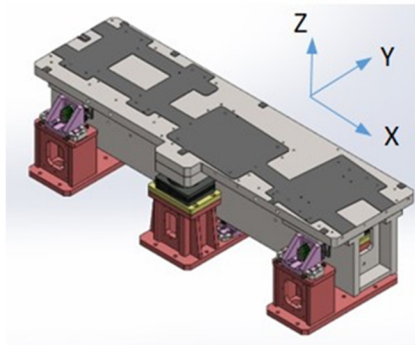
Figure 6: Magnet girder for SPS-II storage ring.
