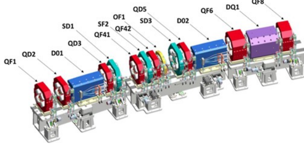
Figure 5: Magnets for half-cell of DTBA lattice.
