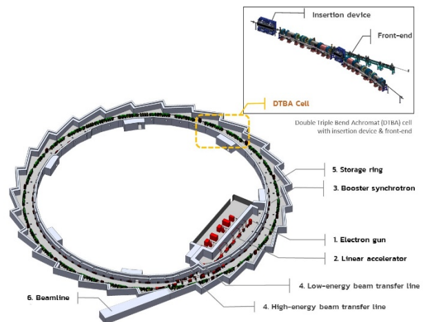
Figure 1: SPS-II accelerator complex.
