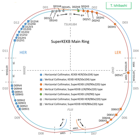
Figure 2: Location of beam collimators in SuperKEKB rings.
