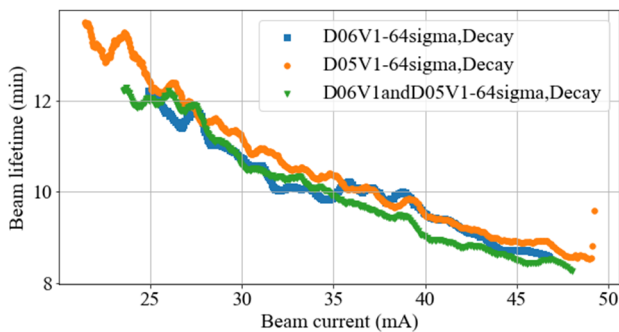
Figure 7: Measured beam lifetime with the effective collimator gap of 64 sigma of the vertical beam size for the D06V1 only, D05V1 only and D06V1 and D05V1 cases.
