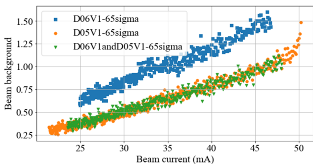
Figure 8: The beam background to the Belle II detector with the same effective vertical gap of the beam collimators. Clearly D05V1 (NLC) works better to reduce the beam background.
