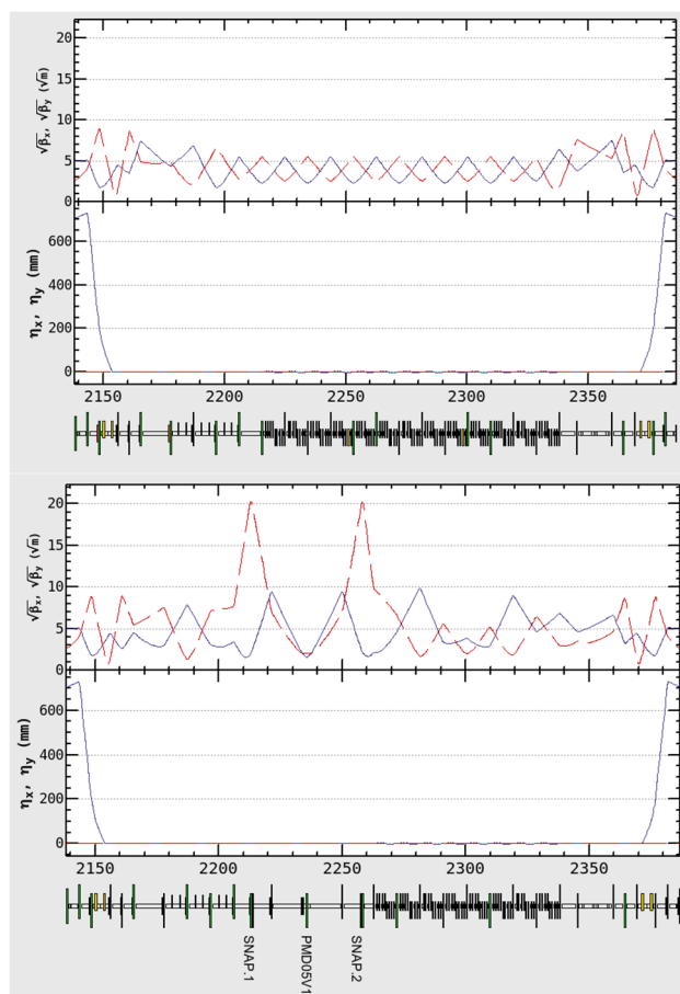
Figure 6: LER beam optics around the NLC. Upper and lower figure show the optics before and after the installation of NLC, respectively.
