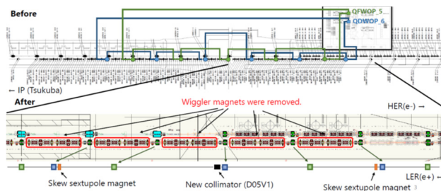
Figure 3: Nonlinear collimator system (NLC) installed at OHO straight section of LER.
