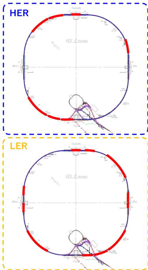
Figure 1: Vacuum-work places of SuperKEKB MR in red line during LS1.
