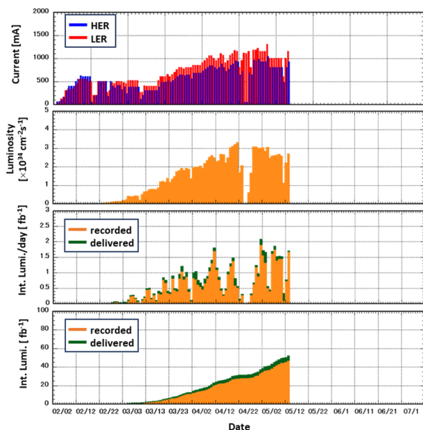
Figure 4: Operation history from the restart after LS1 : beam current (top), peak and daily luminosity (2nd and 3rd), integrated luminosity (bottom).
