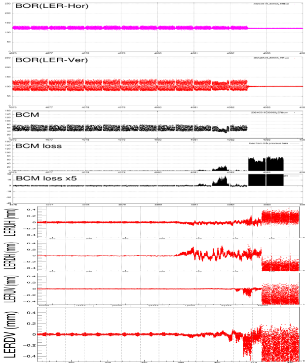
Figure 9: An example of the SBL at LER. Upper figure shows the BOR (H and V, both use the upstream BPM on the bunch feedback system), bunch current information, the loss per turn in bunch current. Lower figures show the reconstructed bunch by bunch position data from bunch feedback processors.
