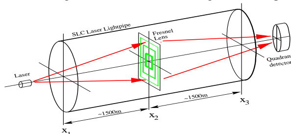
Figure 1: Schematic of the measurement setup.
