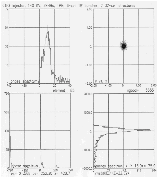
Figure 3: PARMELA results.
