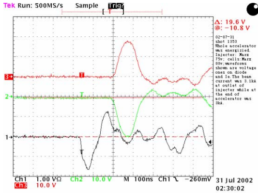
Figure 5: Anode voltage(upper) and cathode voltage(middle)
