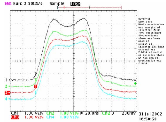
Figure 6: Extracted beam current from injector
