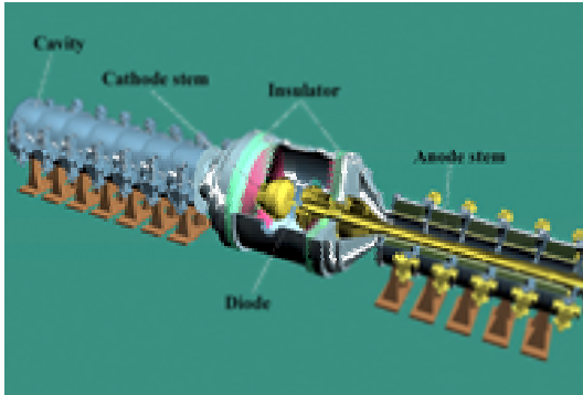
Figure 4: Overview of 3.5MeV injector
