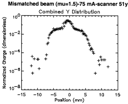
Figure 1: Joined profiles with wire and scraper scanners showing a dynamic range from core to maximum extent of nearly six orders of magnitude (the figure and the caption are from ref. [6]).
