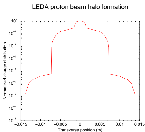
Figure 2: The theoretical transverse charge profile with beam envelope modulation \mu = 1.5 , W = 6.7 MeV, R_0 = 0.0013 m, \Delta R_0 = 0.00065 m, R_m = 0.01393 m, L = 1.1 m, I_b = 0.41 A (proton), f = 0.18 , and \epsilon = 2 mm-mrad.
