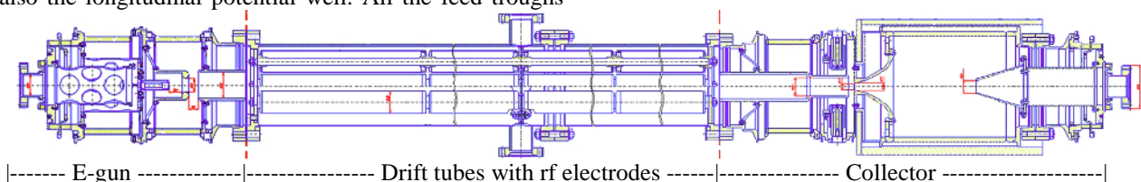
Figure 2: BRIC set-up assembly design, without the solenoids for the electron beam focusing.
