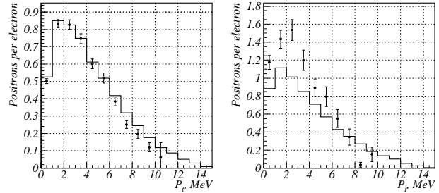
Figure 6: The transverse momentum spectra for 8 mm crystal (left) and 20 mm amorphous (right). Only positrons with energy from 5 to 30 MeV were taken into account. Points is experimental data, histogram \square simulation.
