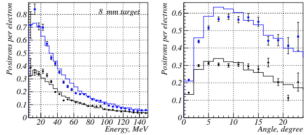
Figure 3: The energy and angular spectra corrected by efficiency for the 8 mm target. E^- = 6 GeV. Boxes \square crystal, points \bullet amorphous target. Histograms \square corresponding simulation.
