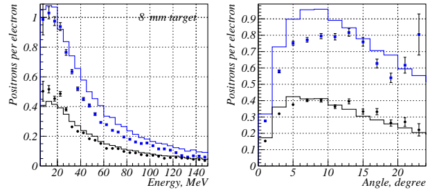
Figure 2: The energy and angular spectra corrected by efficiency for the 8 mm target. E^- = 10 GeV. Boxes \square crystal, points \bullet amorphous target. Histograms \square corresponding simulation.
