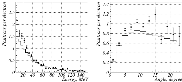
Figure 5: The energy and angular spectra corrected by efficiency for the 20 mm amorphous target. E^- = 10 GeV. Points \bullet experimental data, histogram \square simulation.
