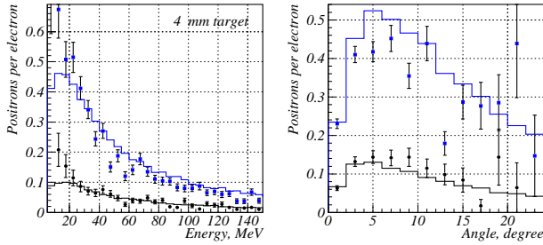
Figure 4: The energy and angular spectra corrected by efficiency. 4 mm target. E^- = 10 GeV. Boxes \square crystal, points \bullet amorphous target. Histograms \square corresponding simulation.
