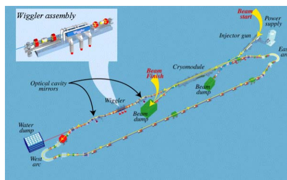
Figure 1. Schematic layout of the Jefferson Lab energy recovering linac IRFEL.
