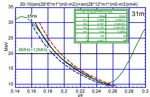
Fig. 12 Composed waveform for phase rotation.
