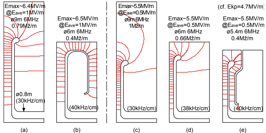
Fig. 9 Phase Rotation Cavity (Single Gap)
