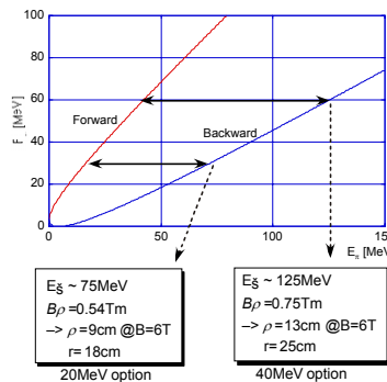
Fig. 3 Muon energy as functions of pion energy.
