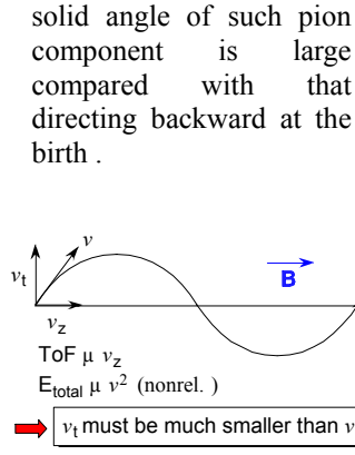
Fig. 6 ToF develops as a function of its longitudinal momentum.
