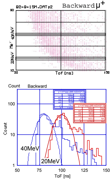
Fig. 7 Energy and longitudinal momentum as a function of ToF after the drift section (25m). Time is measured from the target.
