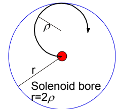
Fig. 4 Motion in a solenoid field and required bore.
