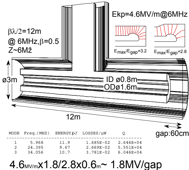
Fig. 10 Phase rotation cavity (Coax type)
