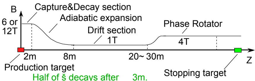
Fig. 2 Magnetic field distribution for PRISM/L
