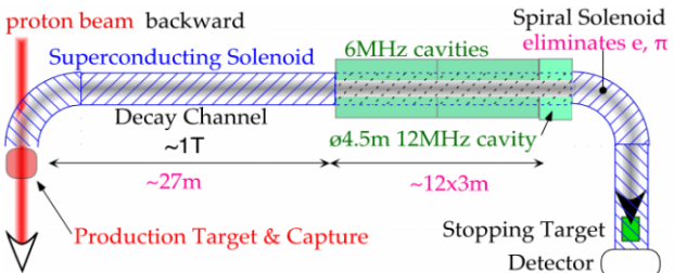
Fig. 11 PRISM/L system
