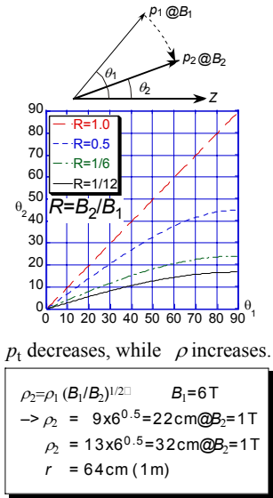
Fig. 5 Adiabatic expansion
