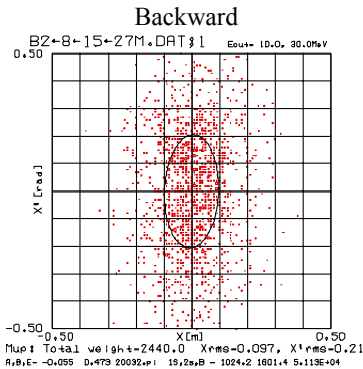
Fig. 8 Phase space at 27m.
