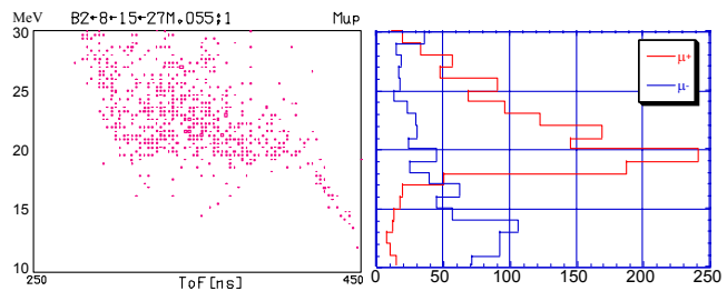
Fig. 13 Muon distributions. Left: energy as a function of ToF, right: projected histogram to the energy axis.
