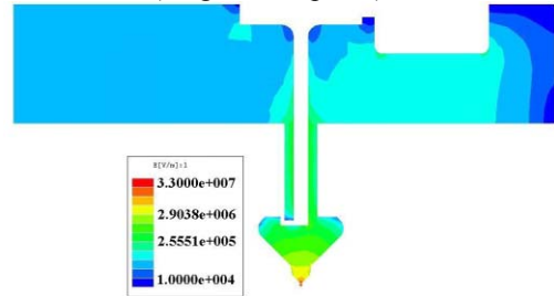
Fig.7 Electric field magnitude in the RFQ and coupler (longitudinal plane)
