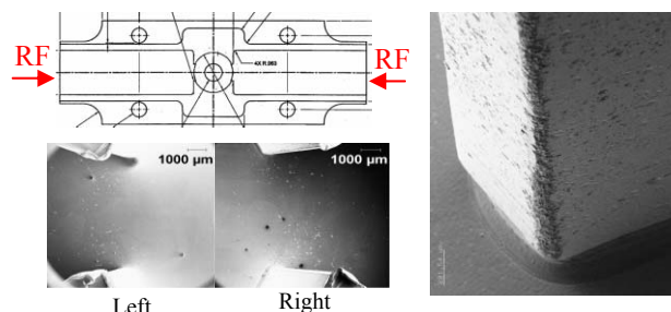
Figure 1: Damaged input coupler of a 0.03 c structure
