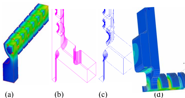
Figure 2. Several couplers with low pulse heating.
