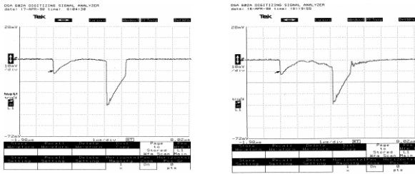
Figure 1: The RF waveform of pulse compressor output power; within temperature control of 45\pm 0.1 °C (left) and beyond temperature control of 45\pm 0.5 °C (right)[2]
