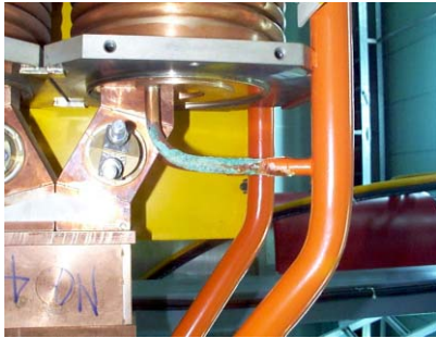
Figure 2: Water leaks in tube joint of SLED system
