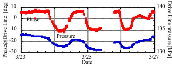
Fig. 4(a) N 2 -gas pressure and driveline phase drift (Feedback off)
