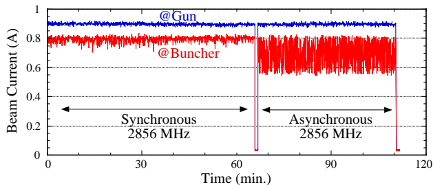
Fig.2 Stability of single-bunched beam
