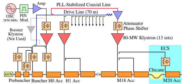
Fig.3 Diagram of improved RF
