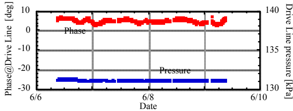
Fig. 4(b) N 2 -gas pressure and driveline phase drift (Feedback on)
