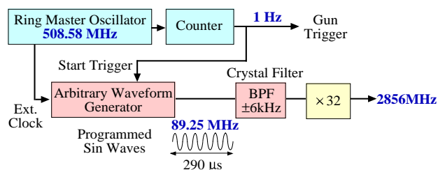
Fig. 1 Block diagram of RF reference generator.
