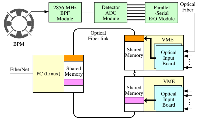
Fig.5 Block diagram of BPM data acquisition system
