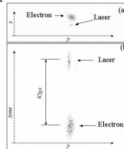
Figure 2: Streak camera images showing the temporal overlap
