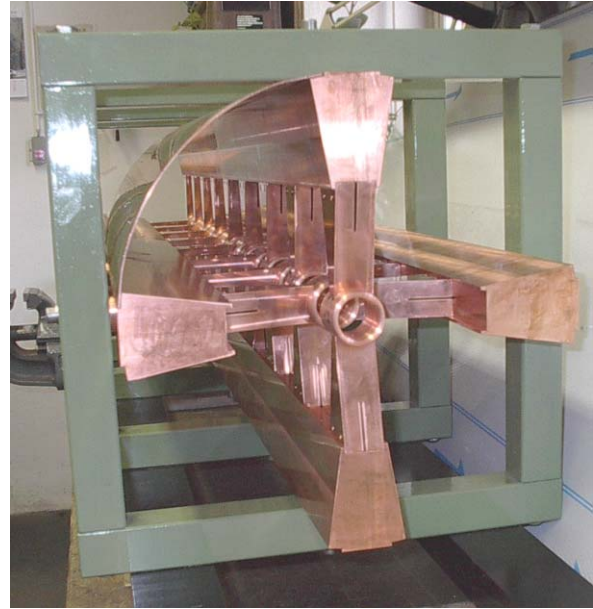
Figure 3: Photo of the CH copper model cavity. The end cells and part of the tank housing is removed
