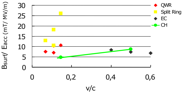
Figure 2: Magnetic to electric field ratio as a function of the particle velocity for different sc cavities. The data were taken from [10].
