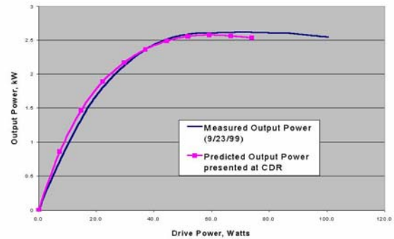
Figure 4: VKP-8290A Transfer Curve
