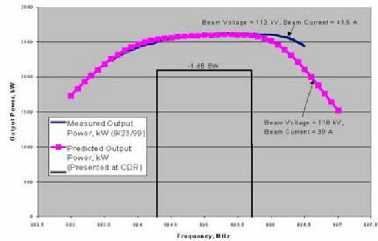
Figure 3: VKP-8290A Bandpass Curve
