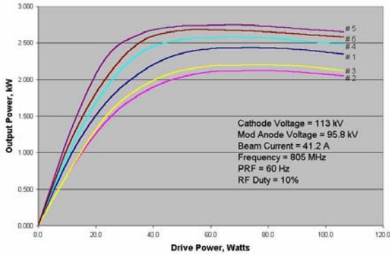
Figure 5: VKP-8290A Transfer Curves at Equally Spaced Mismatch Positions
