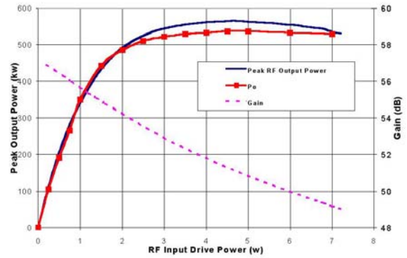
Figure 6: VKP-8291A Transfer Curve
