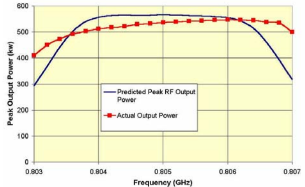
Figure 7: VKP-8291A Predicted Bandpass Curve
